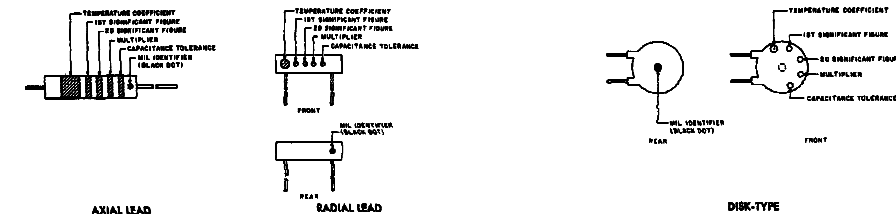
Figure 25. MIL-STD capacitor color code markings.
