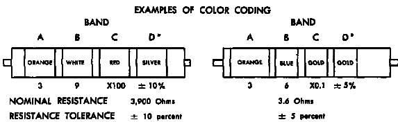
Figure 24. MIL-STD resistor color code markings.
